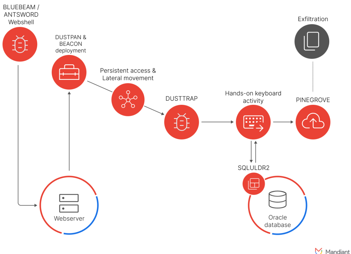
Figure 1: Attack path diagram of observed APT41 attack
